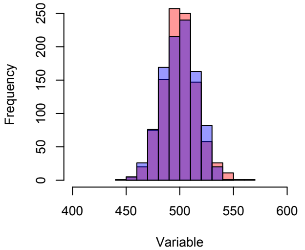
Overlapping Histogram
