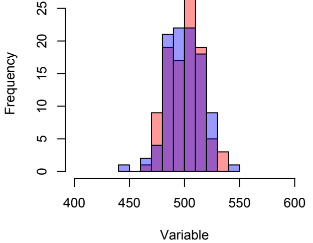
Overlapping Histogram
