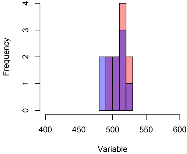
Overlapping Histogram
