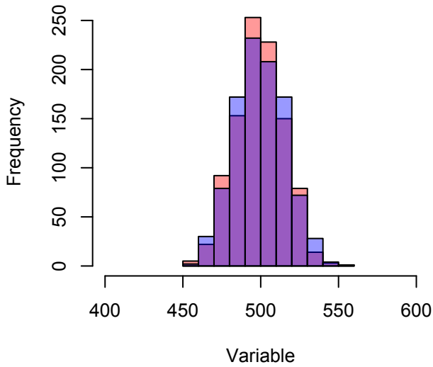
Overlapping Histogram
