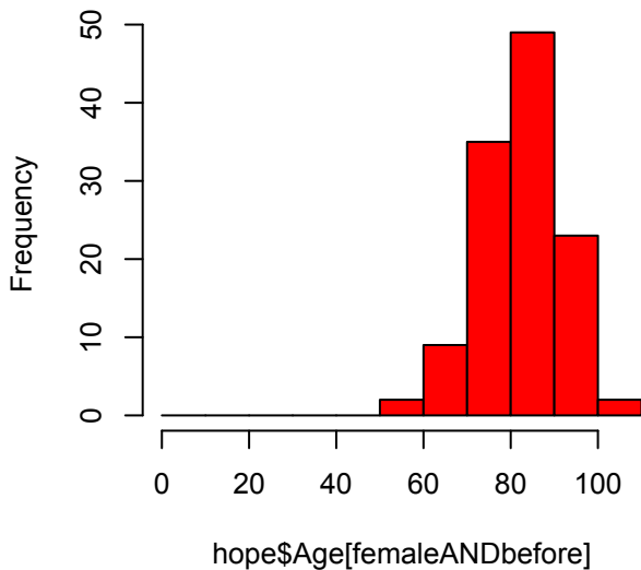
Histogram of hope$Age[femaleANDbefore]
