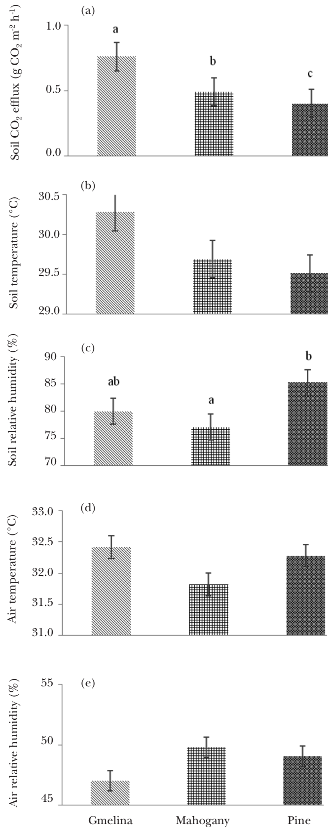
Figure 1 Mean values ( \pm standard errors) across the study period of (a) soil CO 2 efflux, (b) soil temperature, (c) soil relative humidity, (d) air temperature and (e) air relative humidity for gmelina, mahogany and pine study plots; different letters indicate significant differences between tree species
