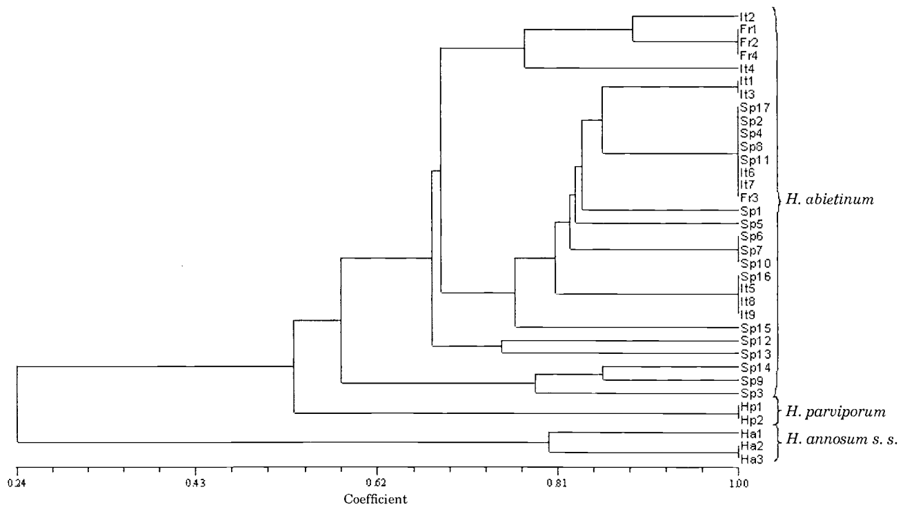
Fig. 1. Dendrogram generated by UPGMA, based on the direct amplification of minisatellite region DNA polymerase chain reaction. The three main clusters of Heterobasidion are shown.
